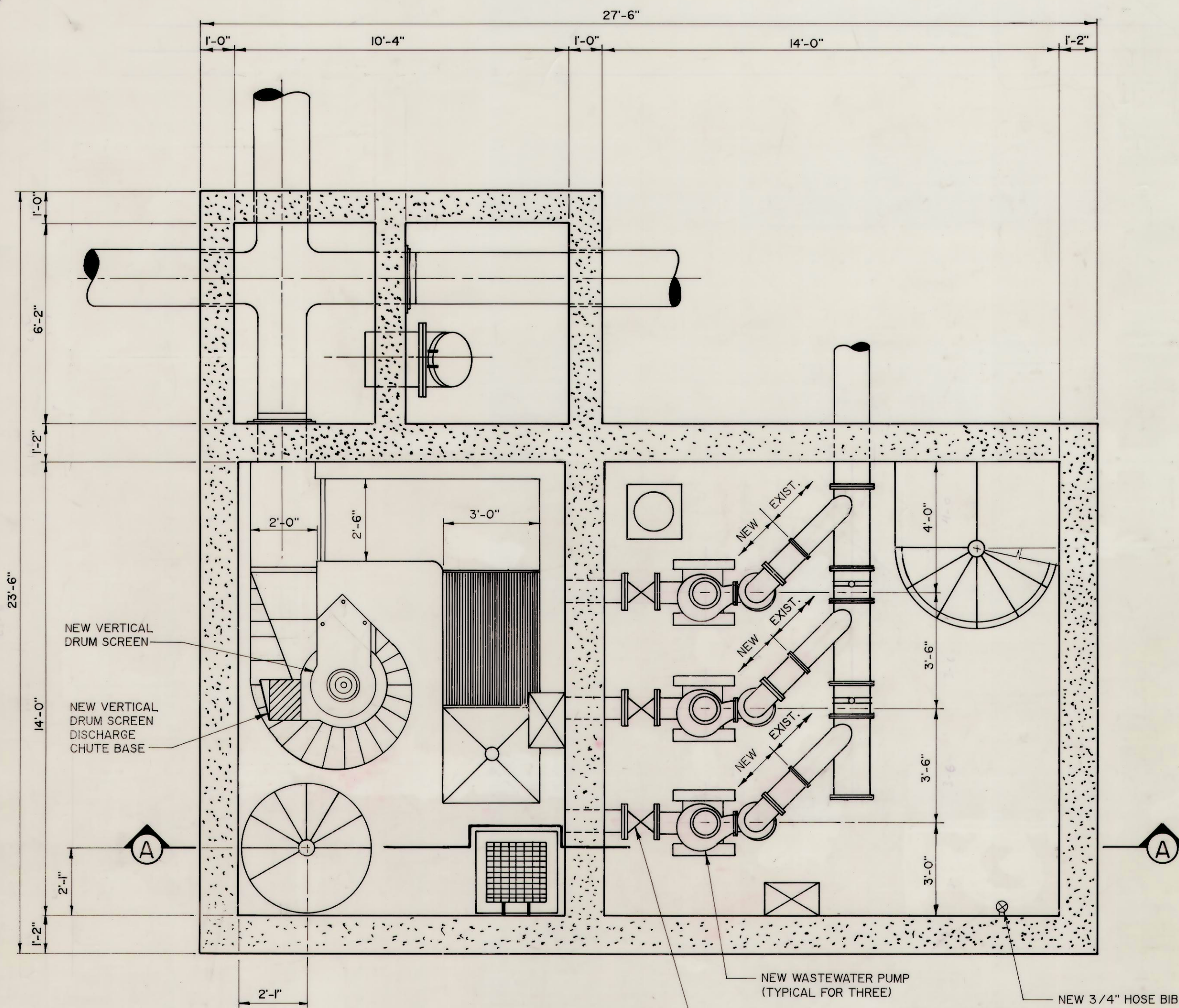
PROPOSED PLAN - LOWER LEVEL EL. 574.56'
